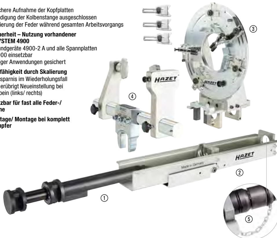
Federspanner 4903/4
